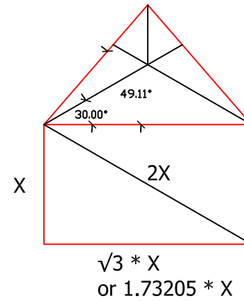
Timber Framing based on Daisy Wheel Geometry
