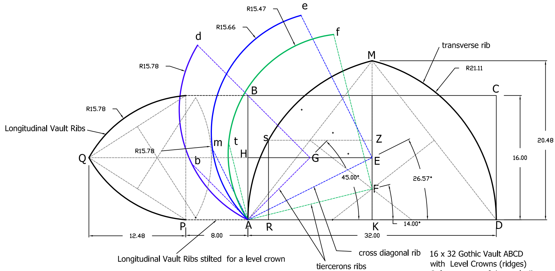
True Gothic Vault with arc's forming all of the ribs from the book
