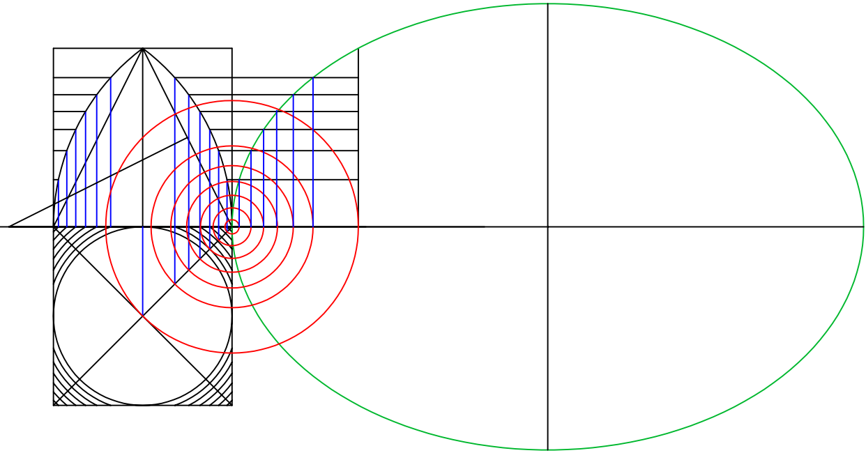
Gothic Cross Vault Elliptical Cross vault diagonals drawn with co-centric circles and ordinates
