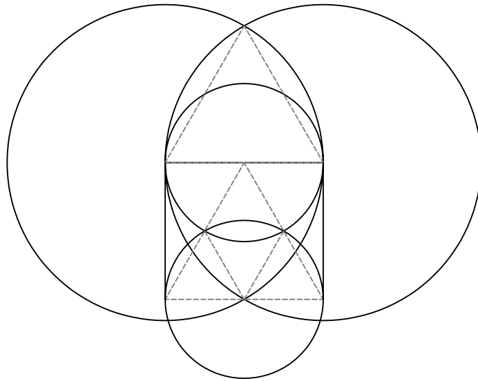
Construction Of Gothic Window with Oculus Based on Euclid's Elements Book 1 Prop 1
