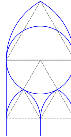
Gothic Window with Oculus
